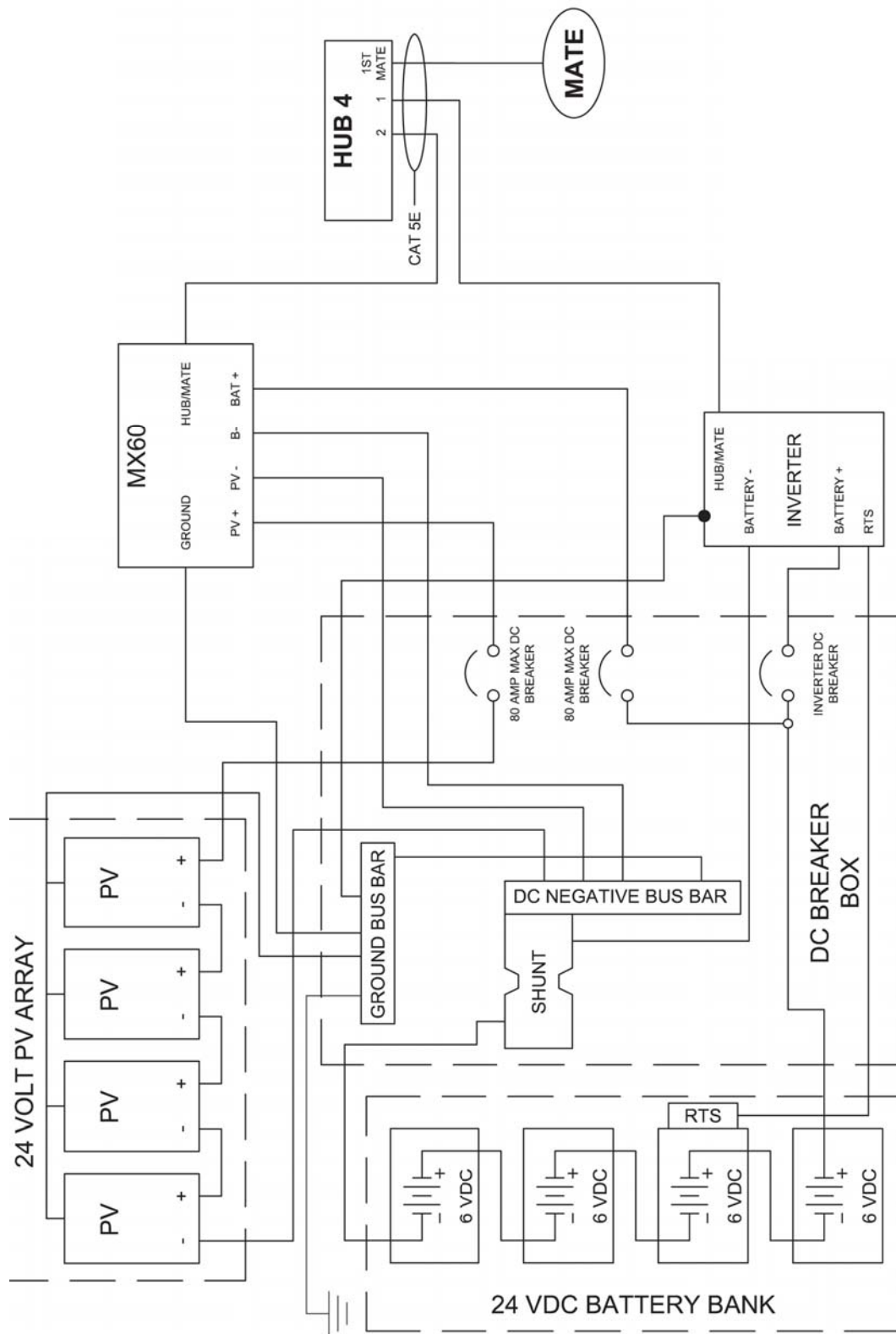
Figure 2 MX60 WIRING DIAGRAM without ground fault protection—the ground conductors tie into the negative.
